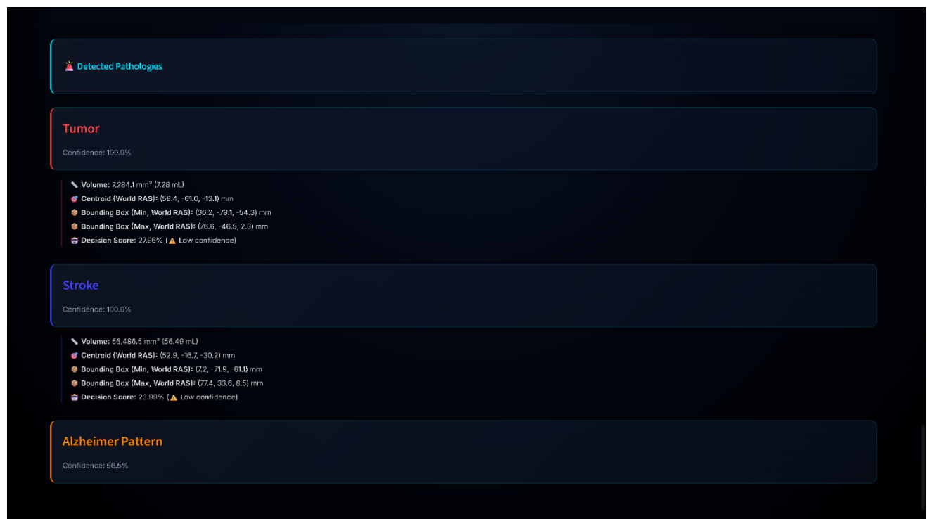
Figure 18 – Detected Pathologies
