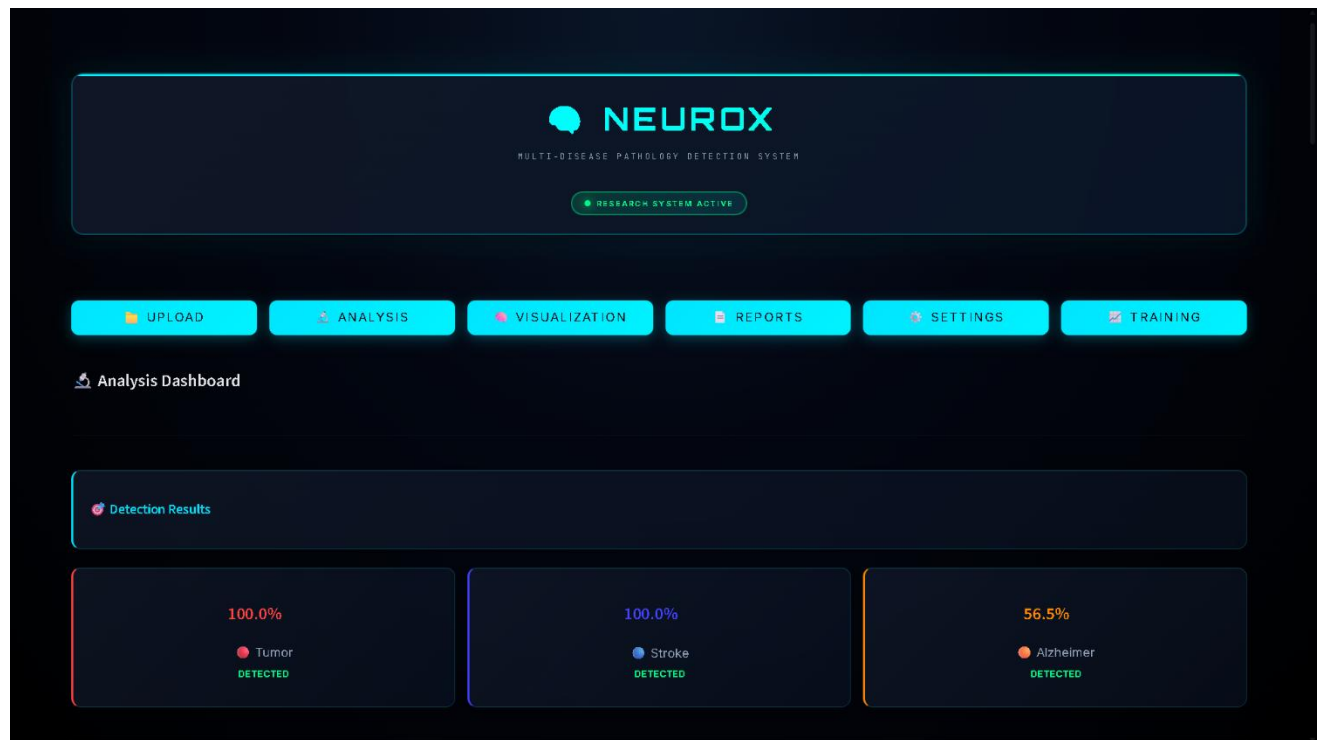
Figure 19 – Analysis Dashboard
